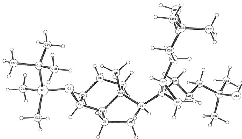
Figure 1. X-ray structure of molecule 5 at 100 °C.
