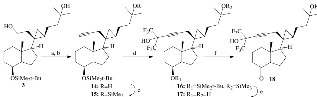
Scheme 3. Reagents: (a) PCC, DCM; (b) MeCON 2 P(O)(OMe) 2 , Na 2 CO 3 , MeOH; (c) TMS-imidazole, DCM; (d) (CF 3 ) 2 CO, BuLi, THF; (e) Bu 4 NF, THF; (f) PDC, DCM.
