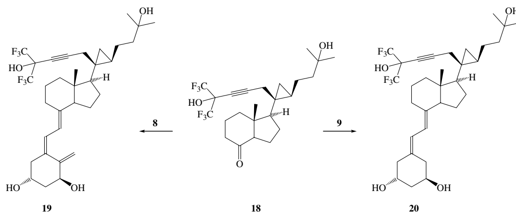
Scheme 3. Reagents: (a) PCC, DCM; (b) MeCON 2 P(O)(OMe) 2 , Na 2 CO 3 , MeOH; (c) TMS-imidazole, DCM; (d) (CF 3 ) 2 CO, BuLi, THF; (e) Bu 4 NF, THF; (f) PDC, DCM.
